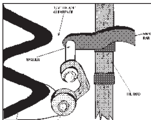
Typical sway bar installed
