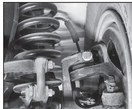
Typical sway bar installed
